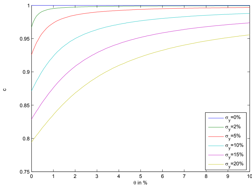
Figure 1: Plot of the function c(\cdot) defined in (14) by varying the mean of the nominal spending process, \theta , and for different standard deviations of the nominal-spending growth process, \sigma_y . \theta and \sigma_y are in percent and at annual rates. \eta = 2.5 , \rho = 0.01 and u^f = 6\% .
